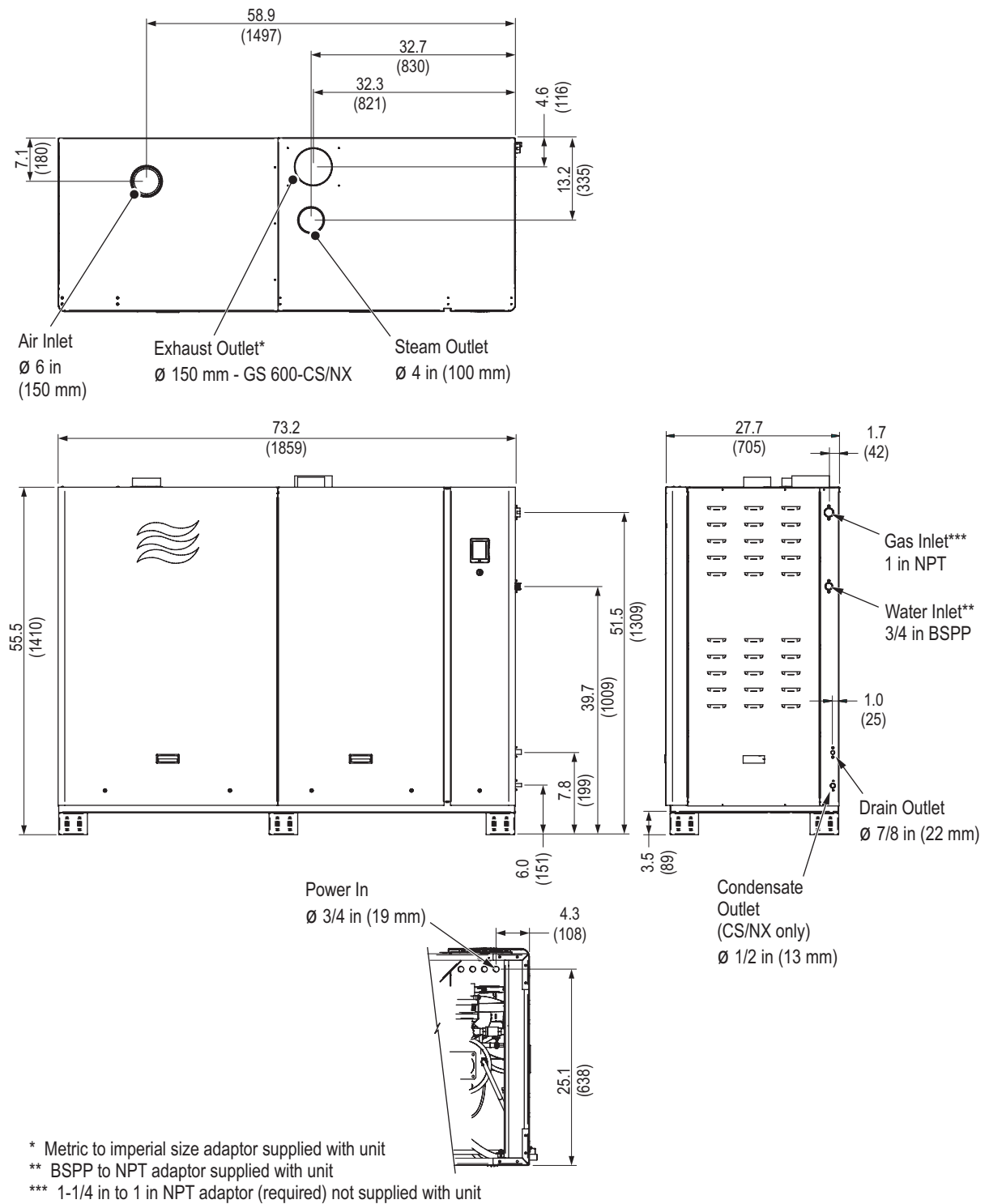
Figure 40: Nortec GS 600
