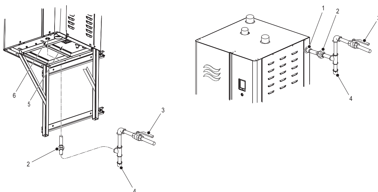
Figure 23: Gas Connection
