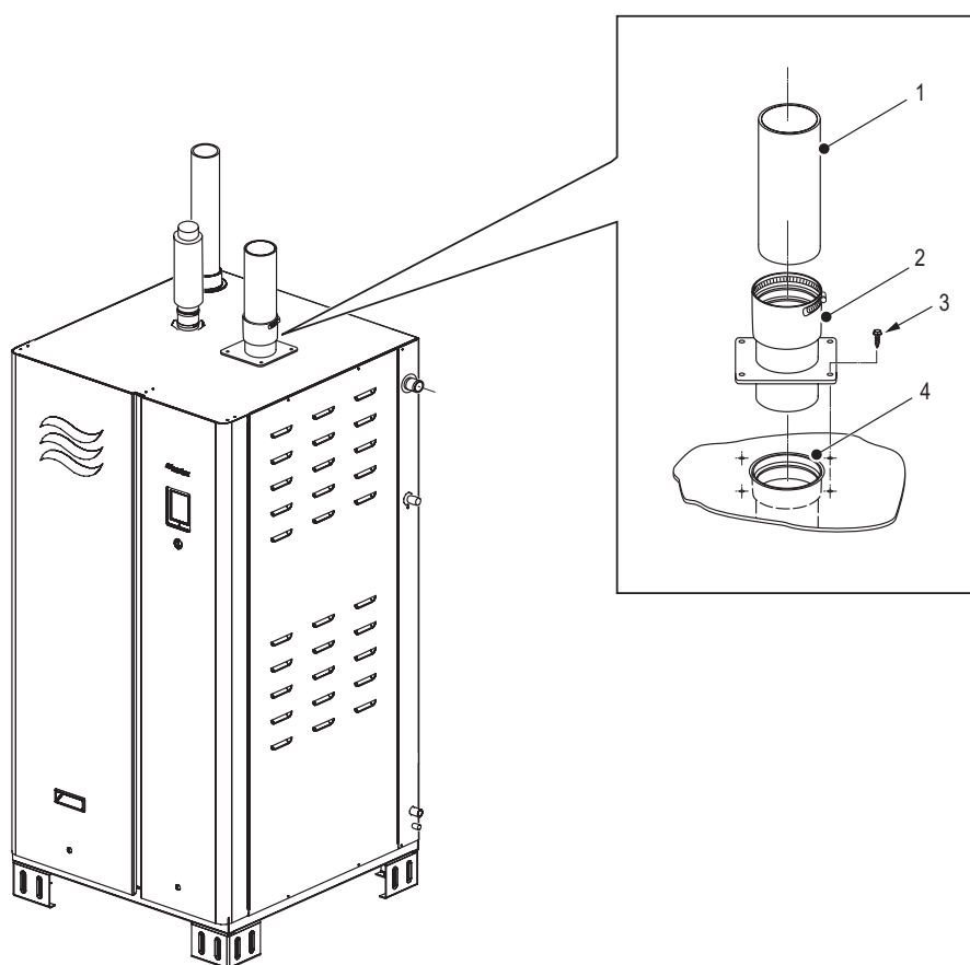
Figure 22: Nortec GS Exhaust Vent Connection – CS/NX Model (Category IV Appliance)
