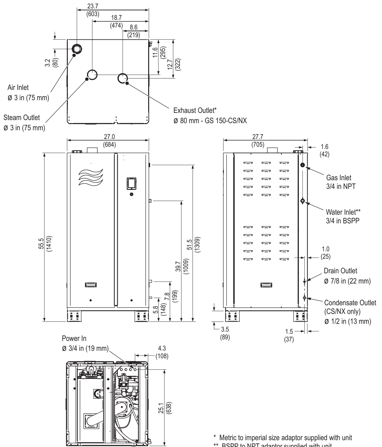
Figure 37: Nortec GS 150
