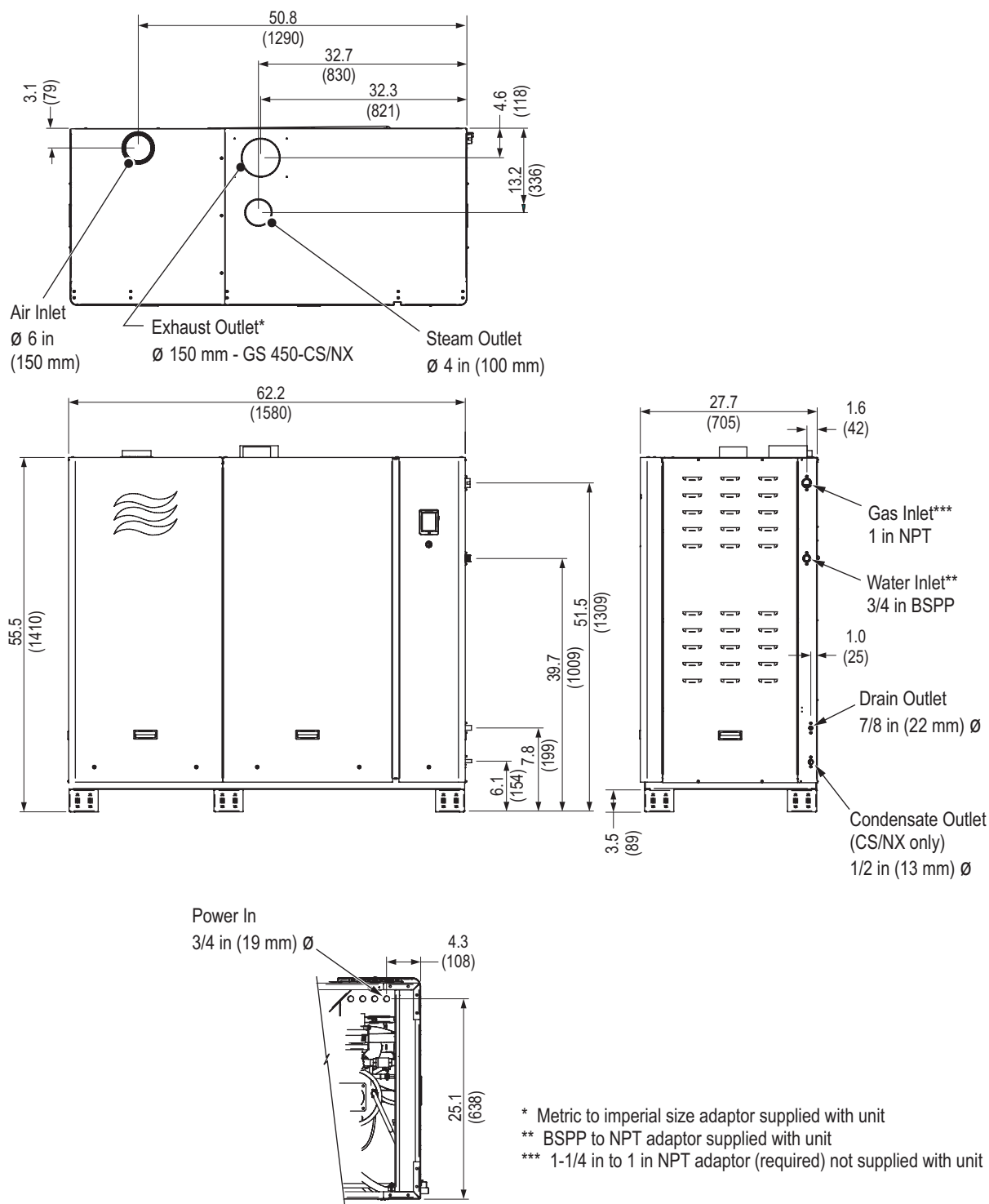
Figure 39: Nortec GS 450
