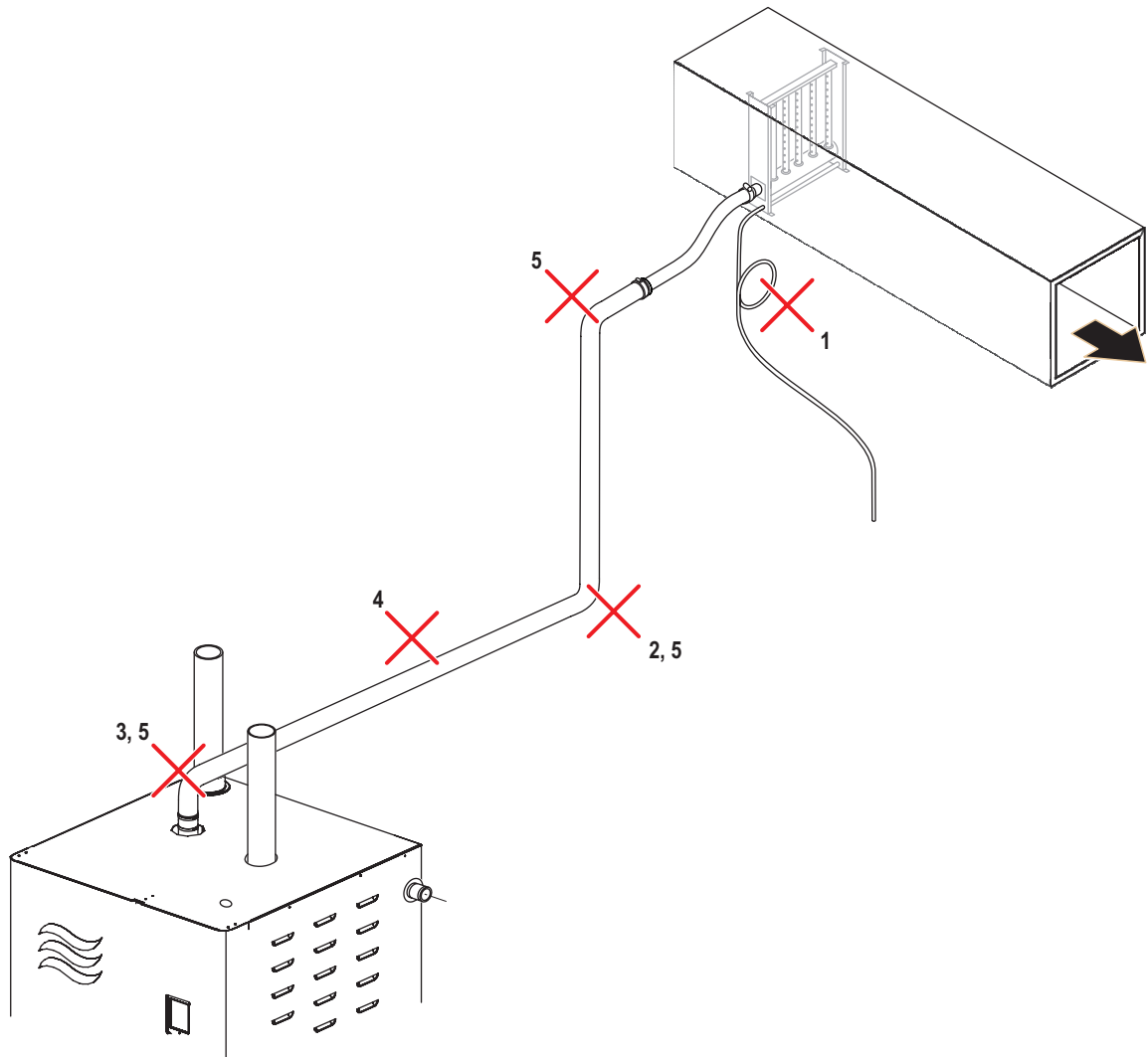
Figure 14: Common Steam and Condensate Line Installation Mistakes
