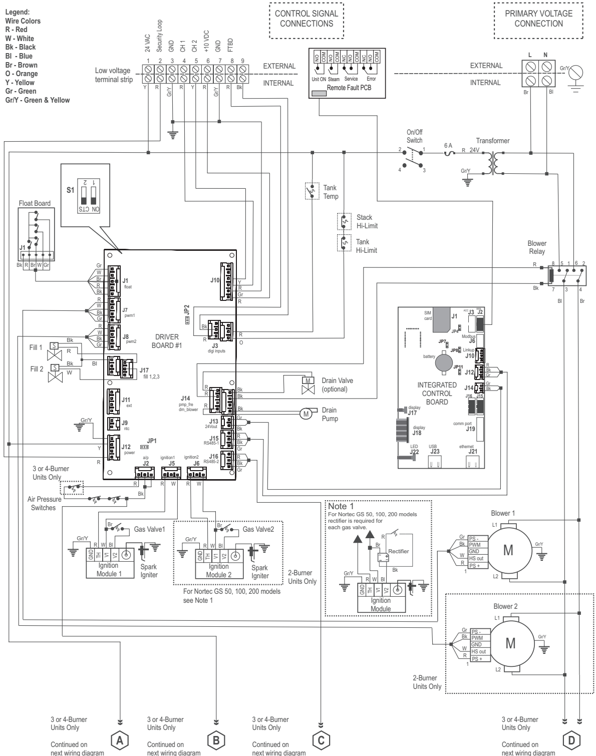
Figure 25: Wiring Diagram - Nortec GS 50/100/150/200/300/450/600
