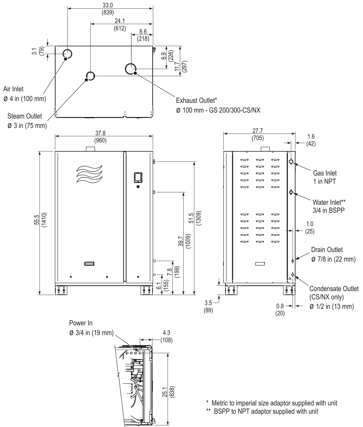
Figure 38: Nortec GS 200/300
