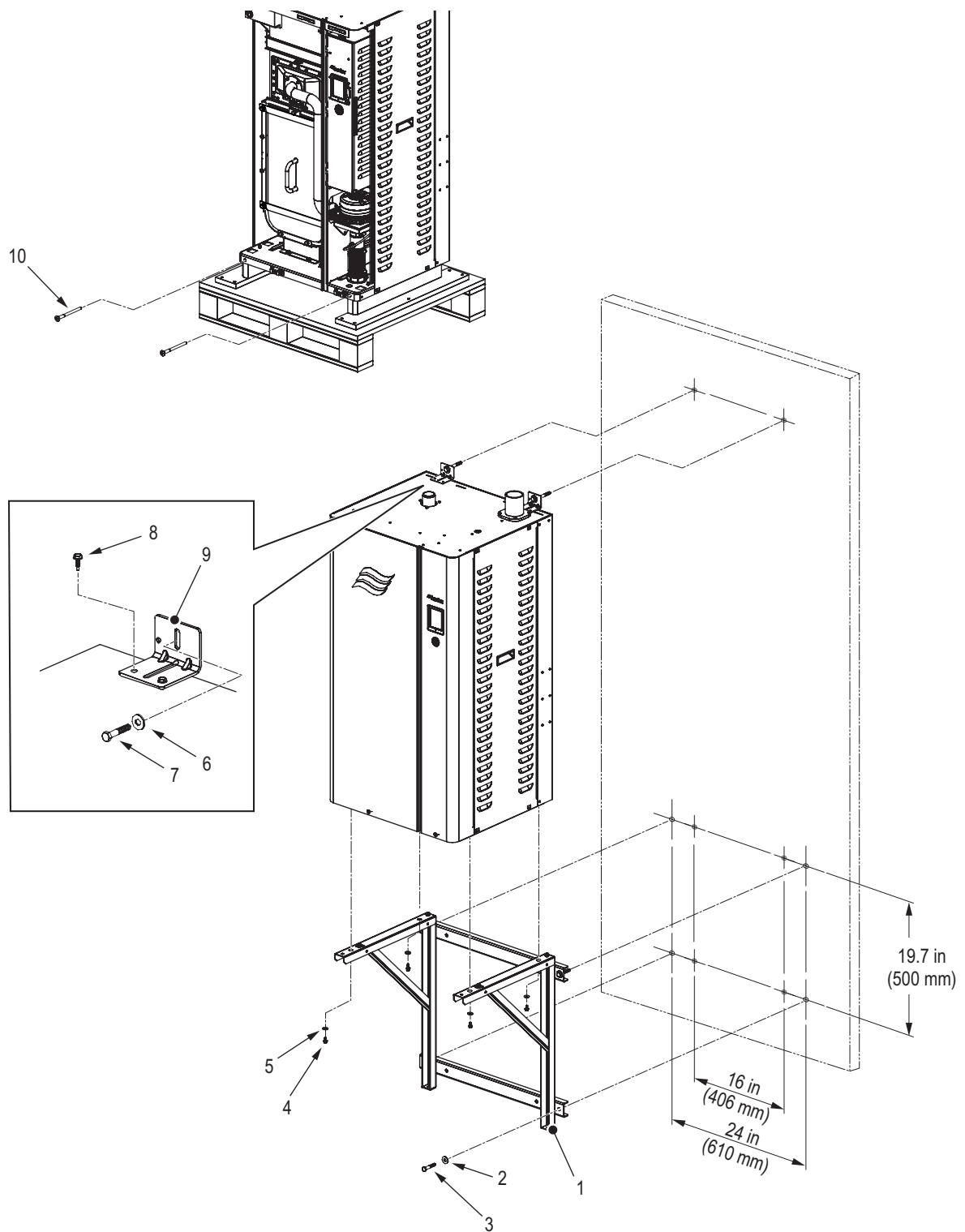
Figure 8: Standard Wall Mounting, Compact Unit Only
