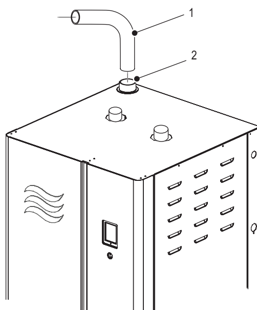
Figure 18: Space Air Installation – GS 150-600
