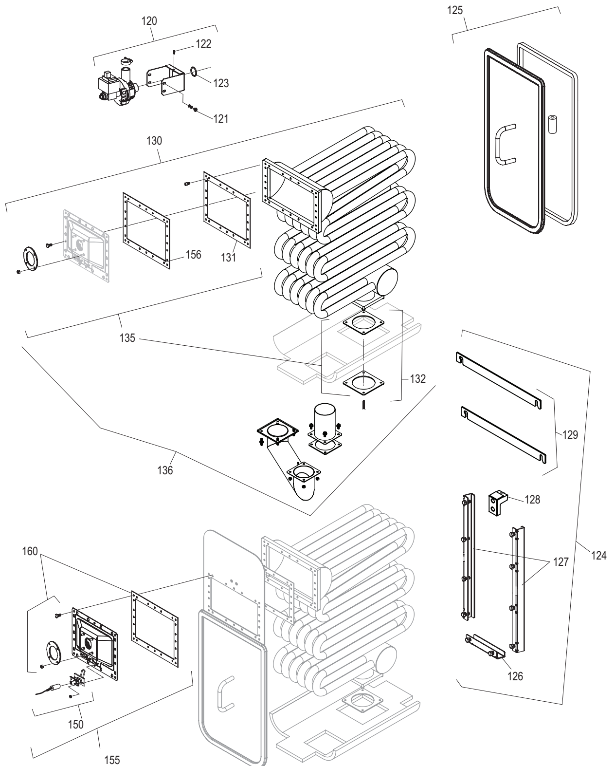
Figure 3: Nortec GS Humidifier, Kit Details
