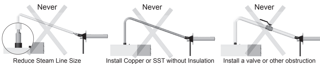
Figure 7: Poor installation examples.
