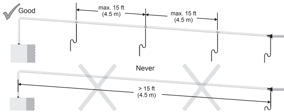
Figure 10: Condensate trap installation locations in long steam line runs.
