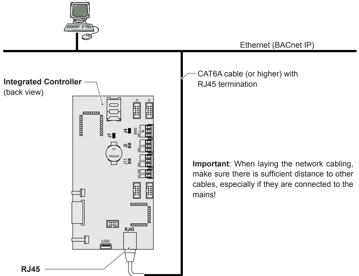
Fig. 1: Principle BACnet IP network
