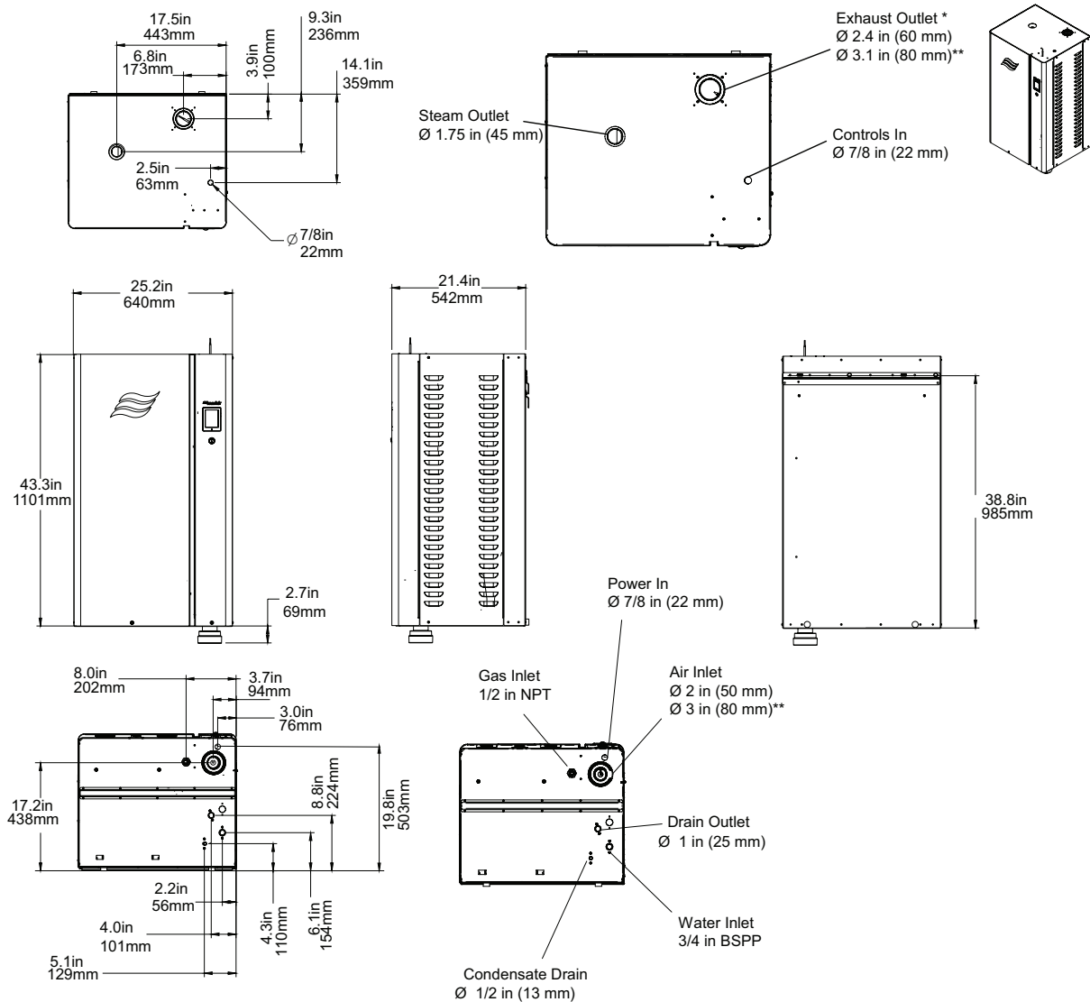
Figure 35: Nortec GS 50/100
