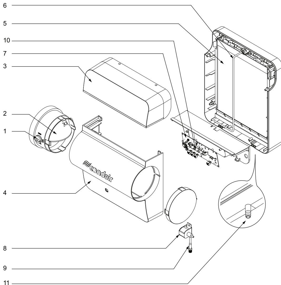
Figure 2 - Composants
