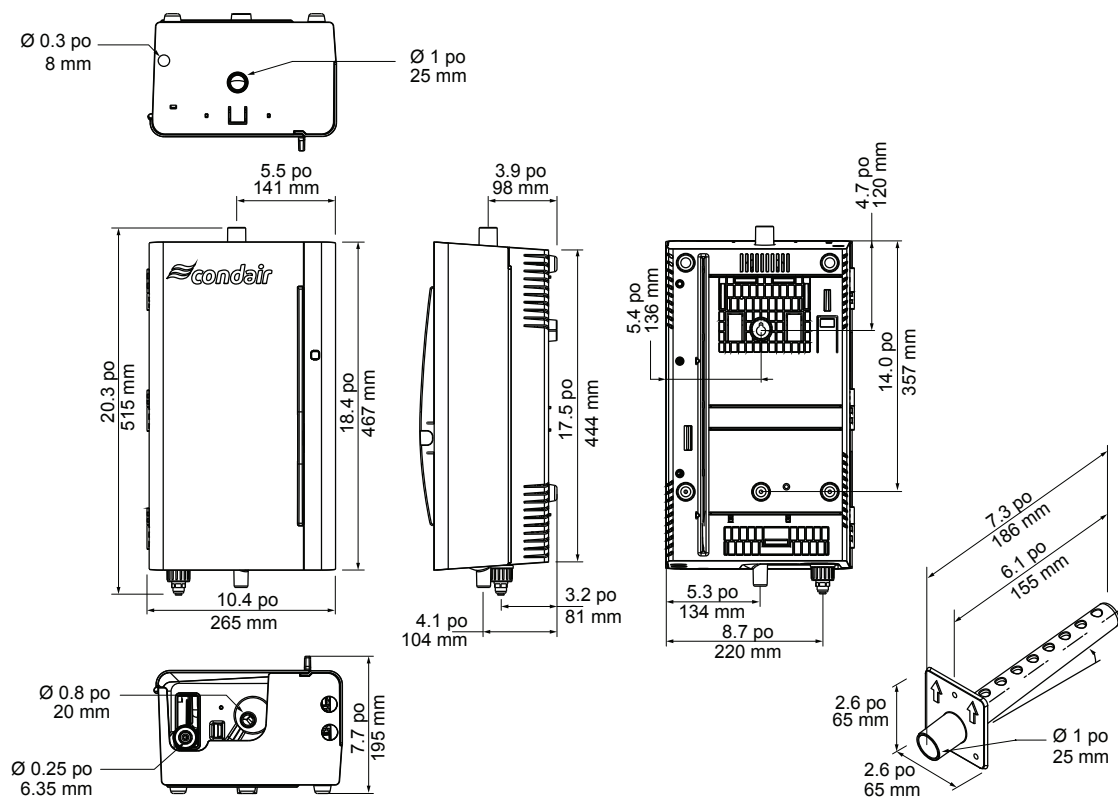
Figure 4 - Dimensions
