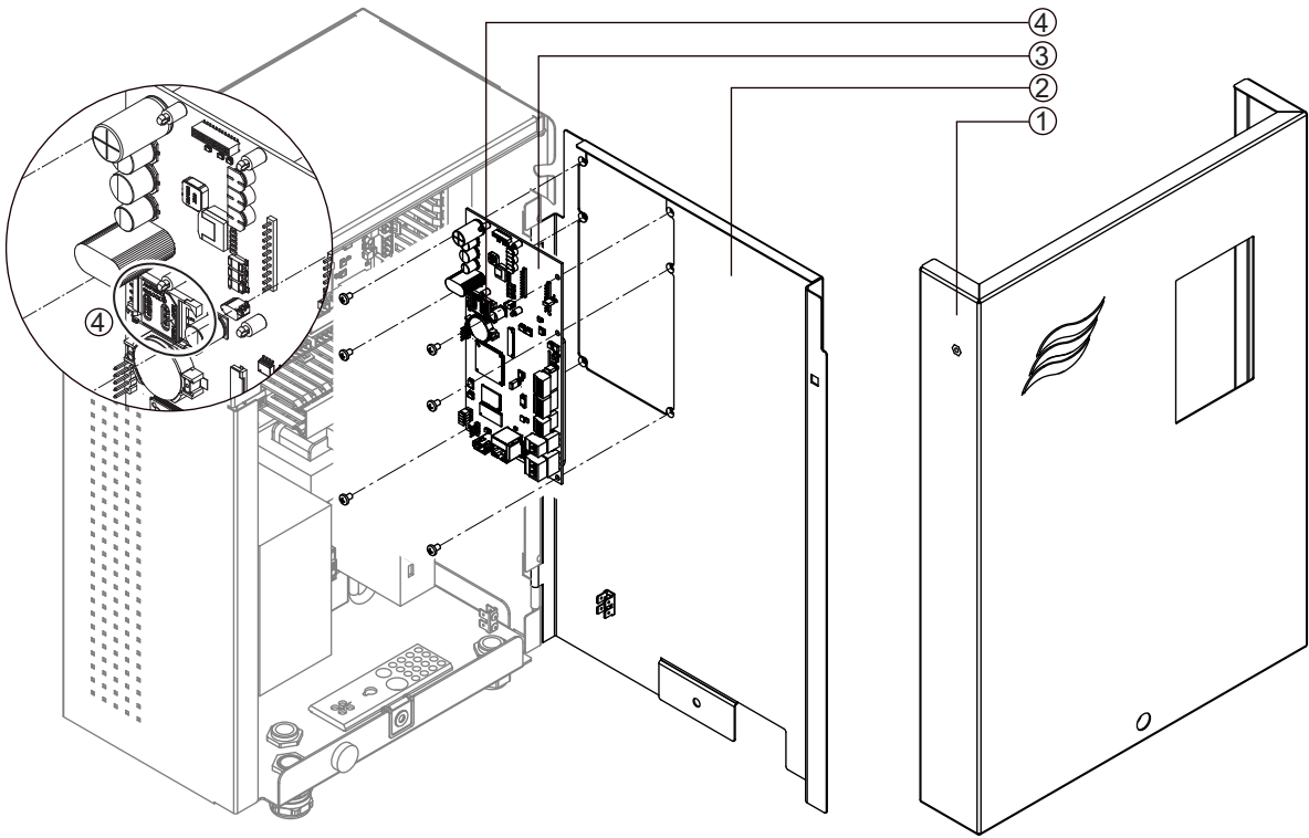
Abb./Fig. 1 Montage Integrated Controller / Installation Integrated Controller
